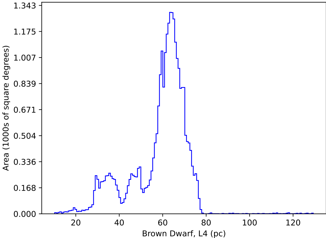
too_elab_heavy_r128_d3_griz_v3.4_10yrs : Brown Dwarf, L4
