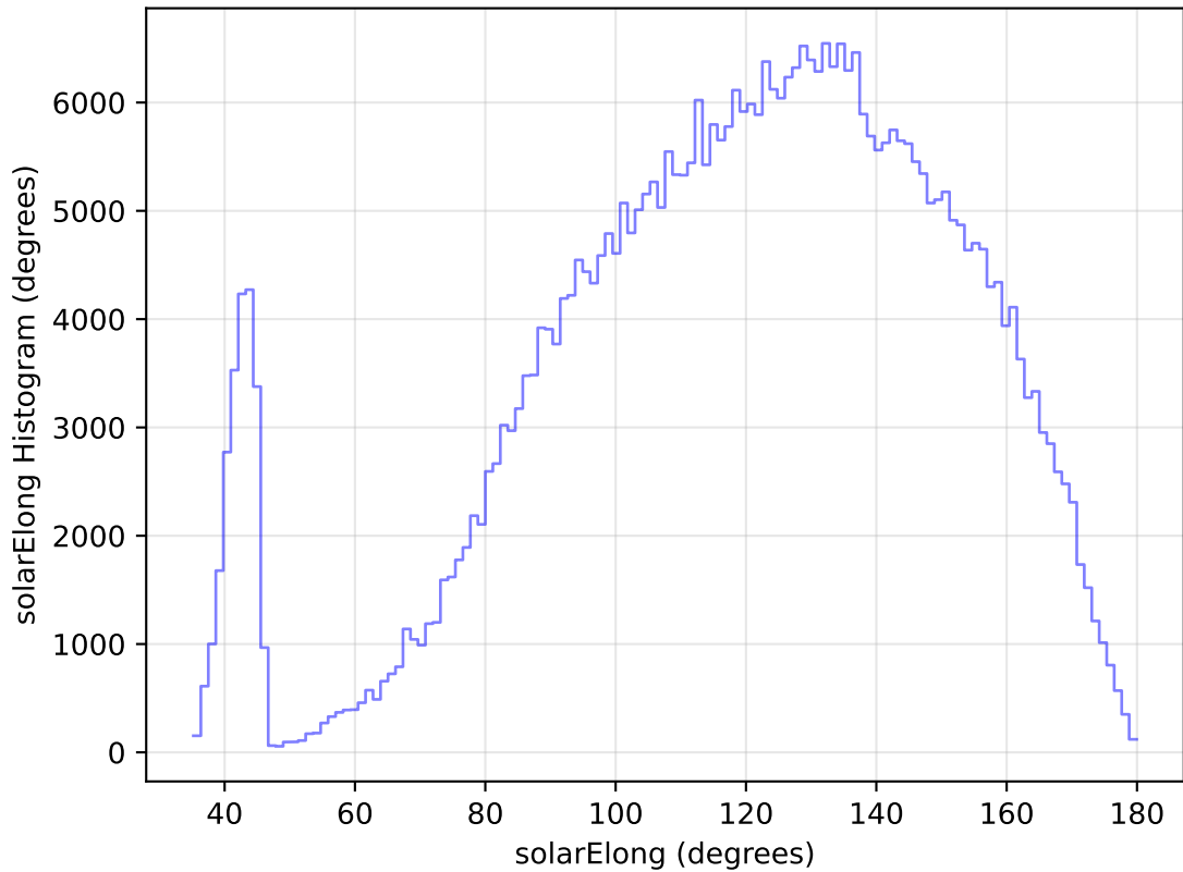
too_elab_heavy_r128_d3_griz_v3.4_10yrs WFD z band: solarElong Histogram
