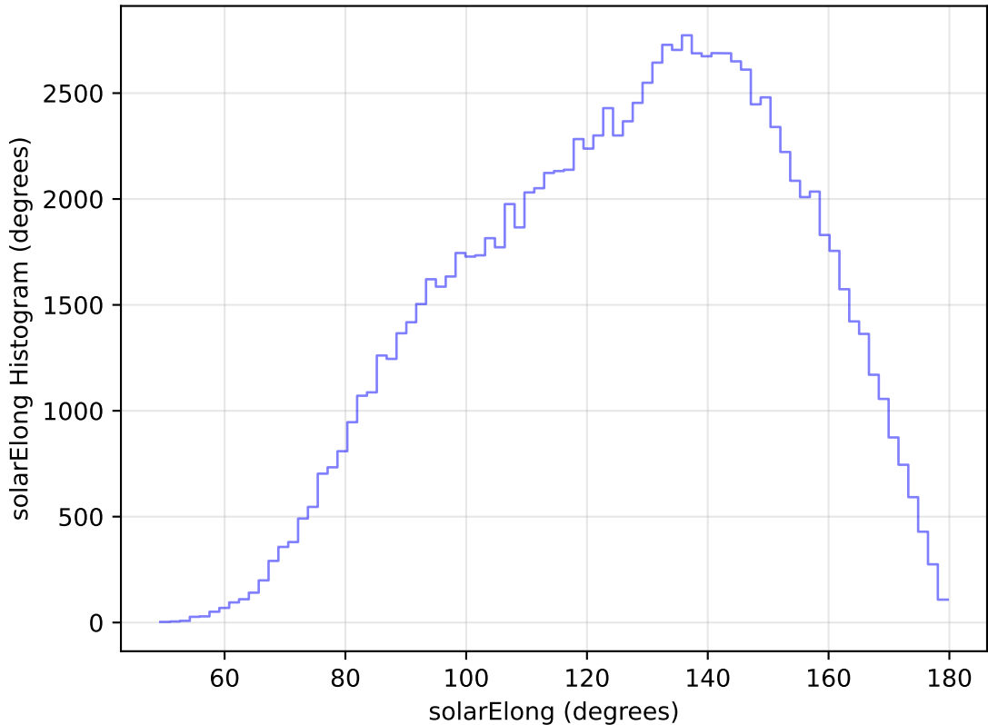
too_elab_heavy_r128_d3_griz_v3.4_10yrs WFD u band: solarElong Histogram
