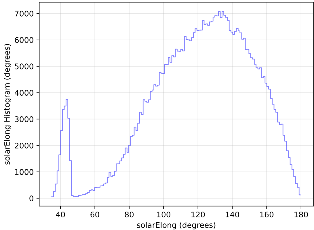
too_elab_heavy_r128_d3_griz_v3.4_10yrs WFD i band: solarElong Histogram
