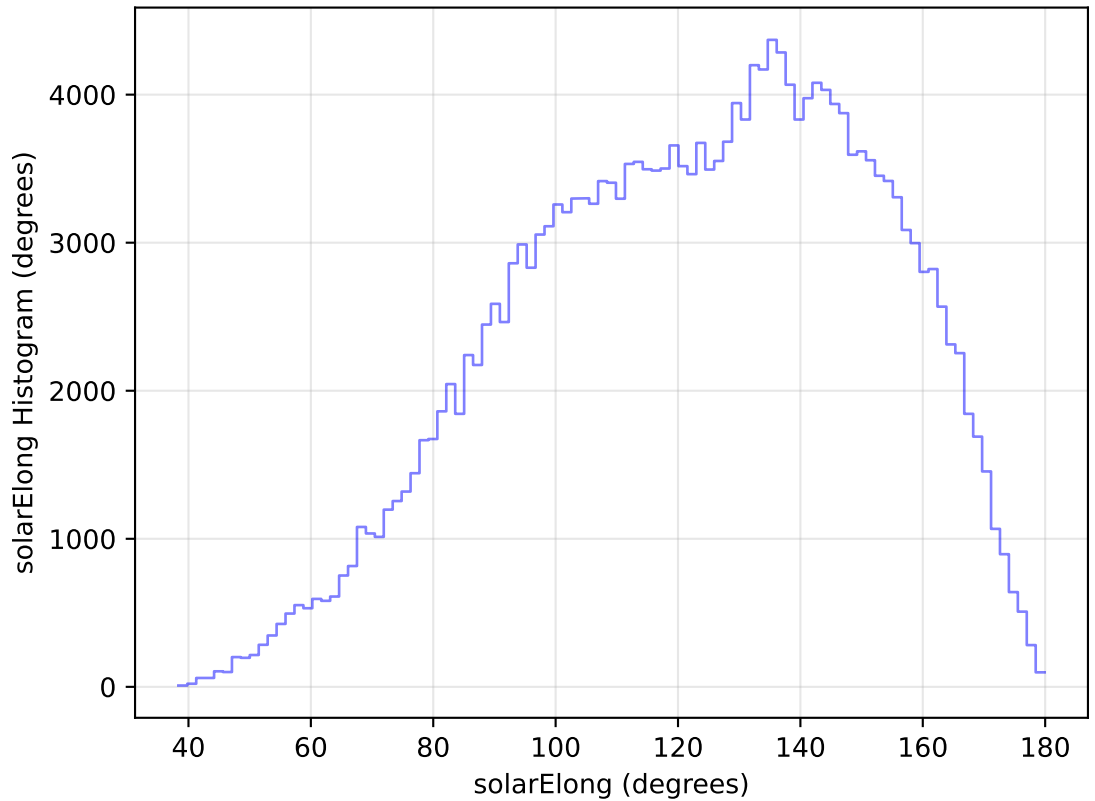
too_elab_heavy_r128_d3_griz_v3.4_10yrs WFD g band: solarElong Histogram
