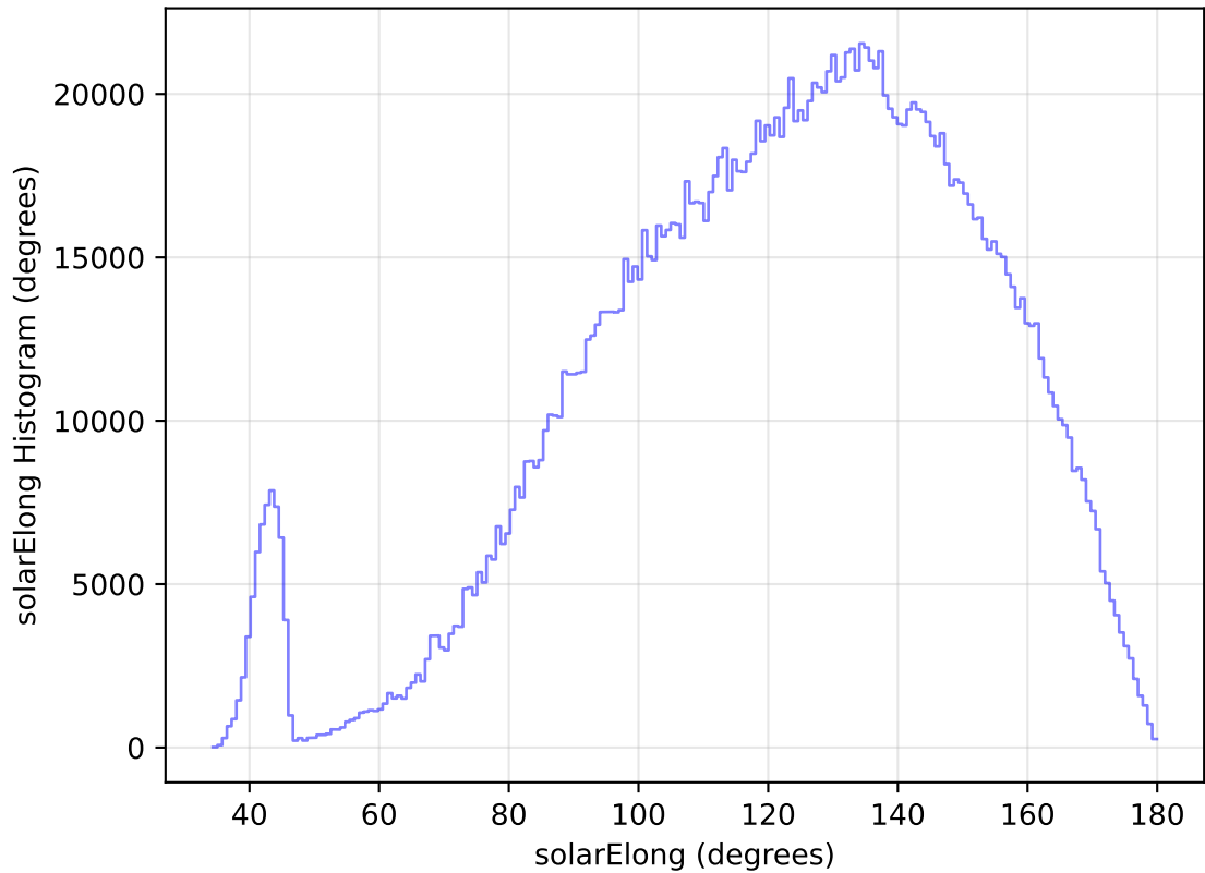
too_elab_heavy_r128_d3_griz_v3.4_10yrs WFD all bands: solarElong Histogram
