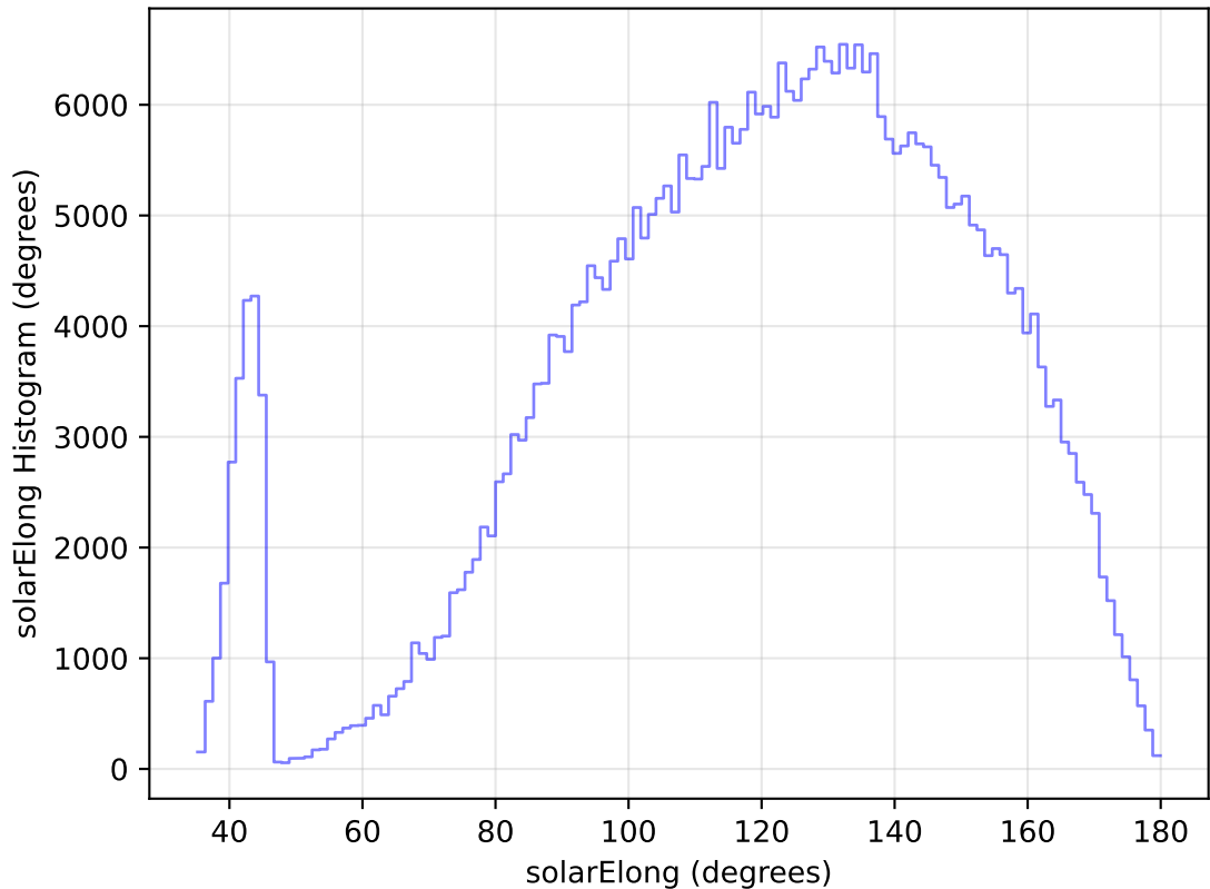
too_elab_heavy_r128_d3_griz_v3.4_10yrs All sky z band: solarElong Histogram
