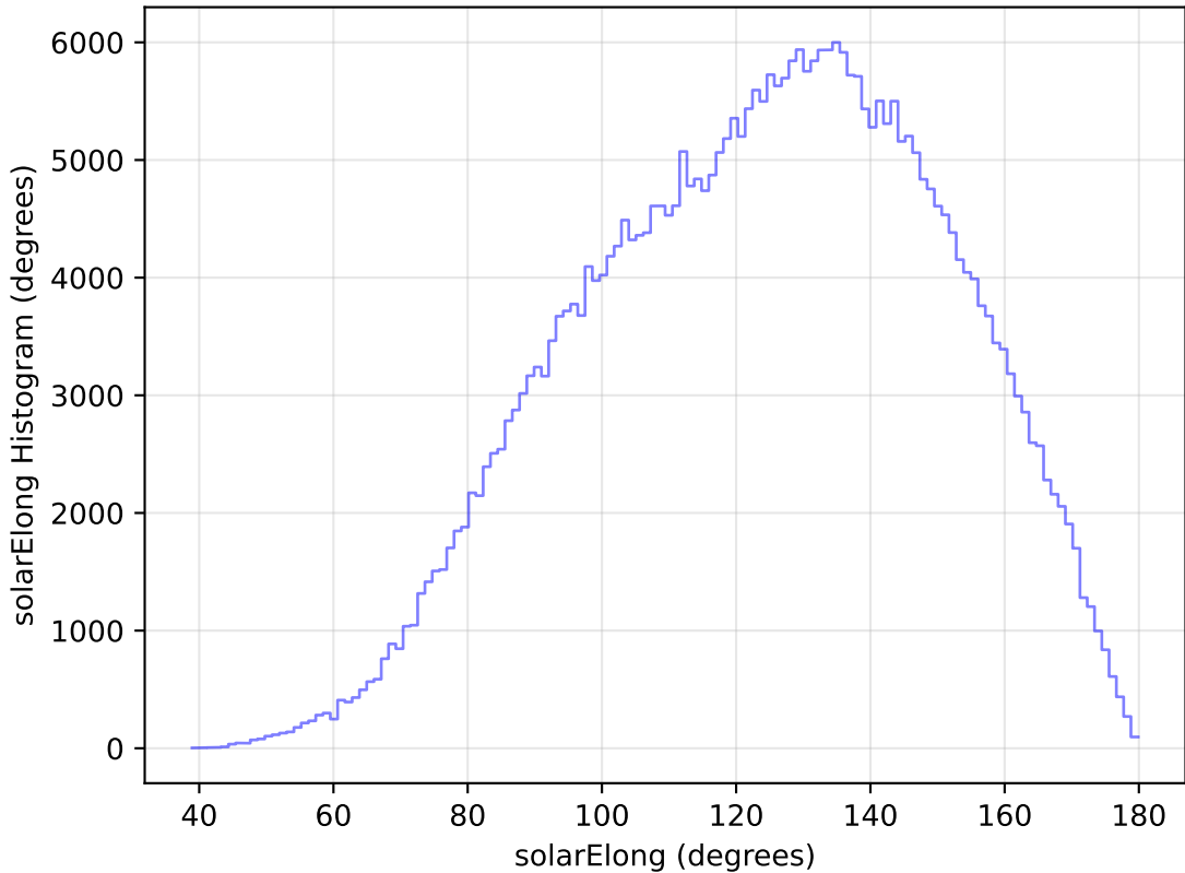
too_elab_heavy_r128_d3_griz_v3.4_10yrs All sky y band: solarElong Histogram
