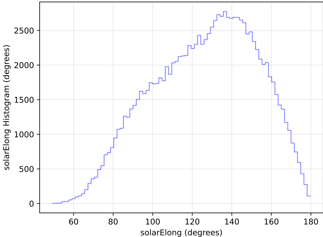
too_elab_heavy_r128_d3_griz_v3.4_10yrs All sky u band: solarElong Histogram
