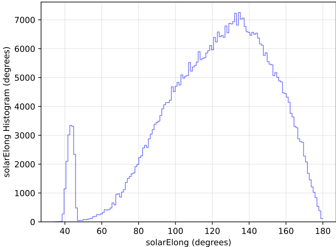
too_elab_heavy_r128_d3_griz_v3.4_10yrs All sky r band: solarElong Histogram
