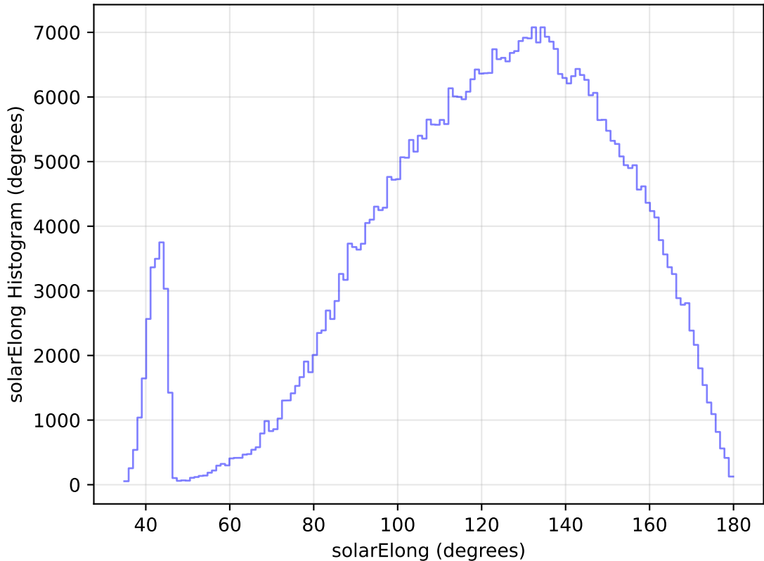
too_elab_heavy_r128_d3_griz_v3.4_10yrs All sky i band: solarElong Histogram
