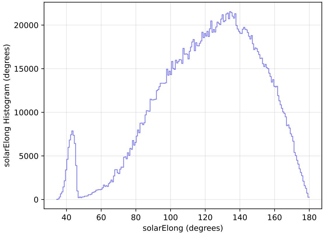
too_elab_heavy_r128_d3_griz_v3.4_10yrs All sky all bands: solarElong Histogram
