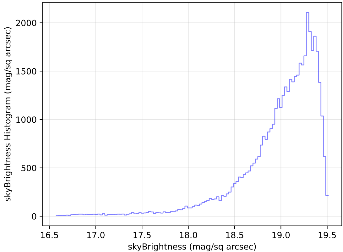
too_elab_heavy_r128_d3_griz_v3.4_10yrs Yr 1 z band: skyBrightness Histogram
