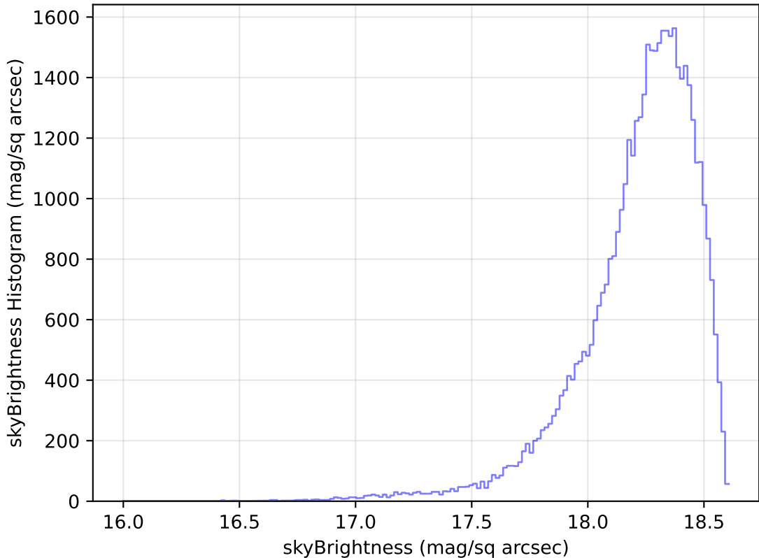
too_elab_heavy_r128_d3_griz_v3.4_10yrs Yr 1 y band: skyBrightness Histogram
