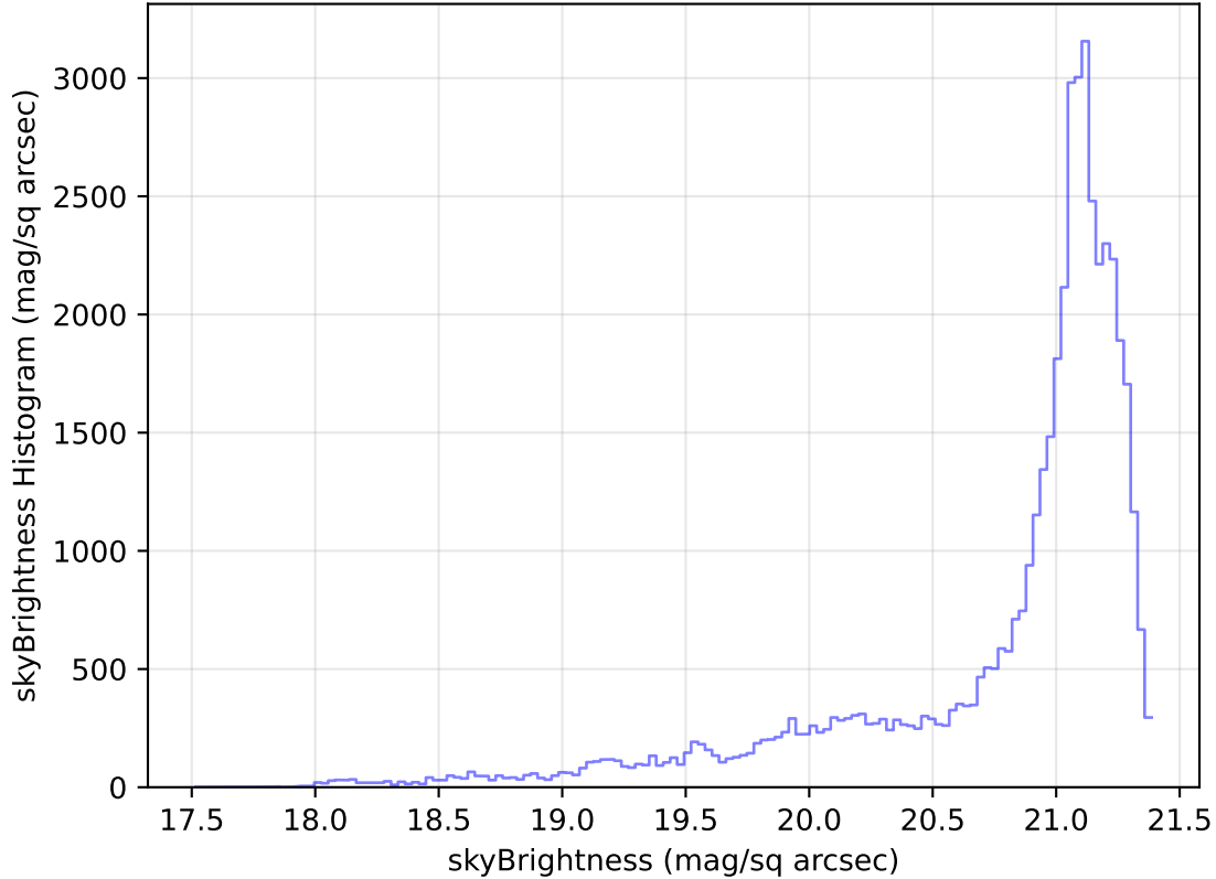
too_elab_heavy_r128_d3_griz_v3.4_10yrs Yr 1 r band: skyBrightness Histogram
