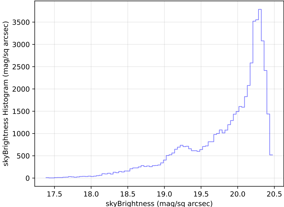
too_elab_heavy_r128_d3_griz_v3.4_10yrs Yr 1 i band: skyBrightness Histogram
