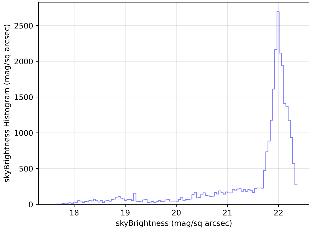
too_elab_heavy_r128_d3_griz_v3.4_10yrs Yr 1 g band: skyBrightness Histogram
