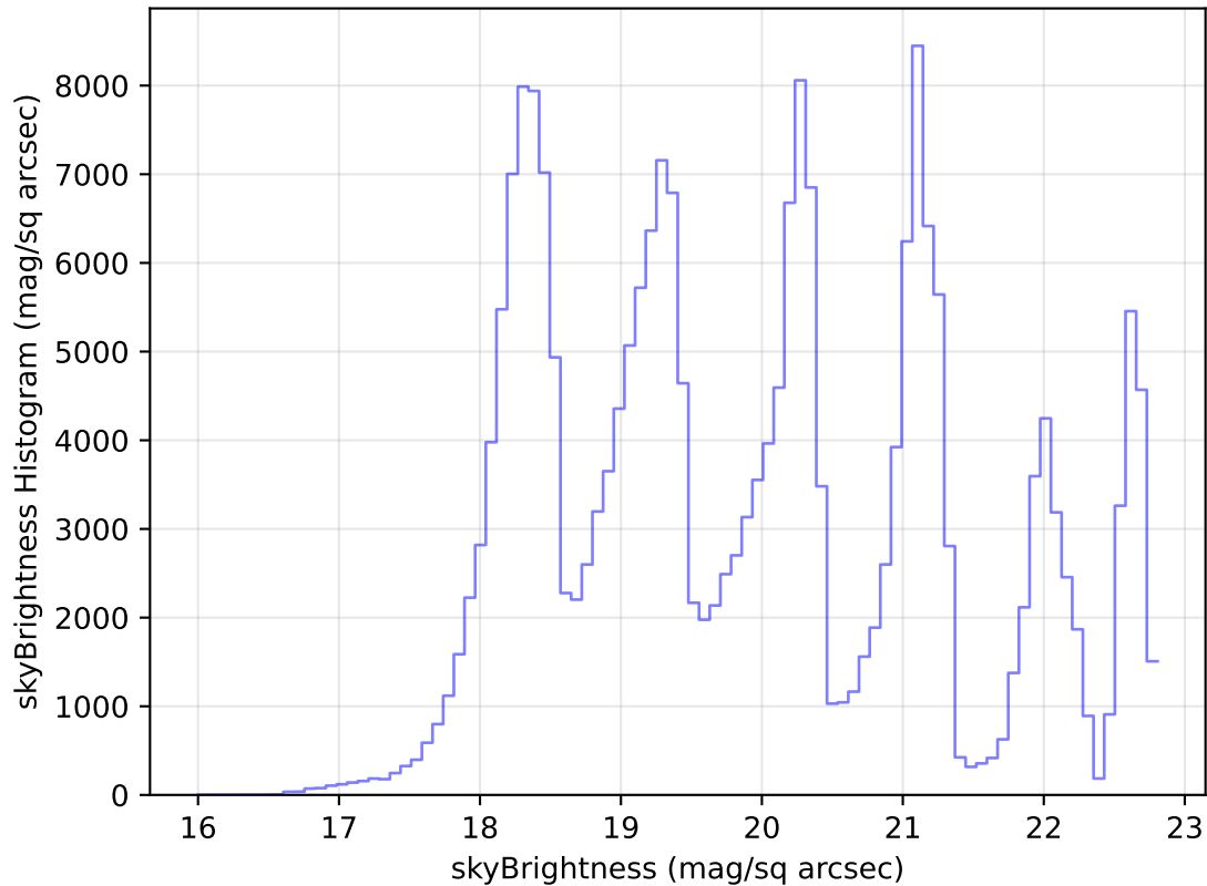
too_elab_heavy_r128_d3_griz_v3.4_10yrs Yr 1 all bands: skyBrightness Histogram
