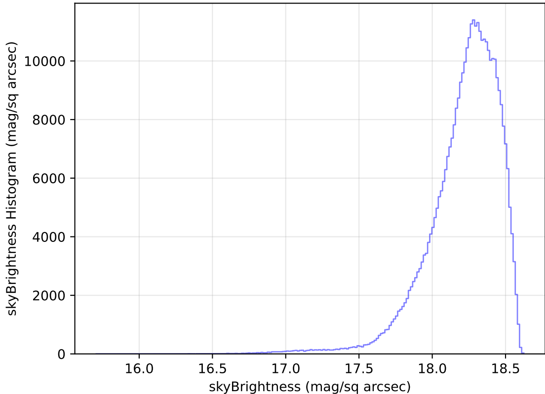
too_elab_heavy_r128_d3_griz_v3.4_10yrs WFD y band: skyBrightness Histogram
