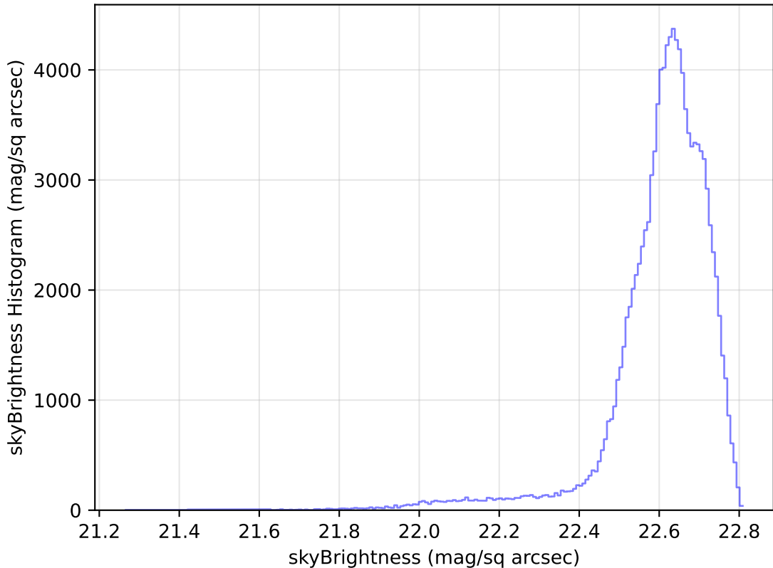
too_elab_heavy_r128_d3_griz_v3.4_10yrs WFD u band: skyBrightness Histogram
