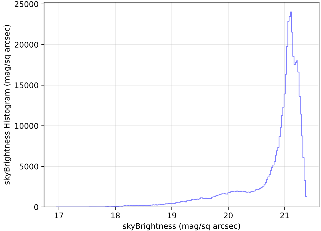
too_elab_heavy_r128_d3_griz_v3.4_10yrs WFD r band: skyBrightness Histogram
