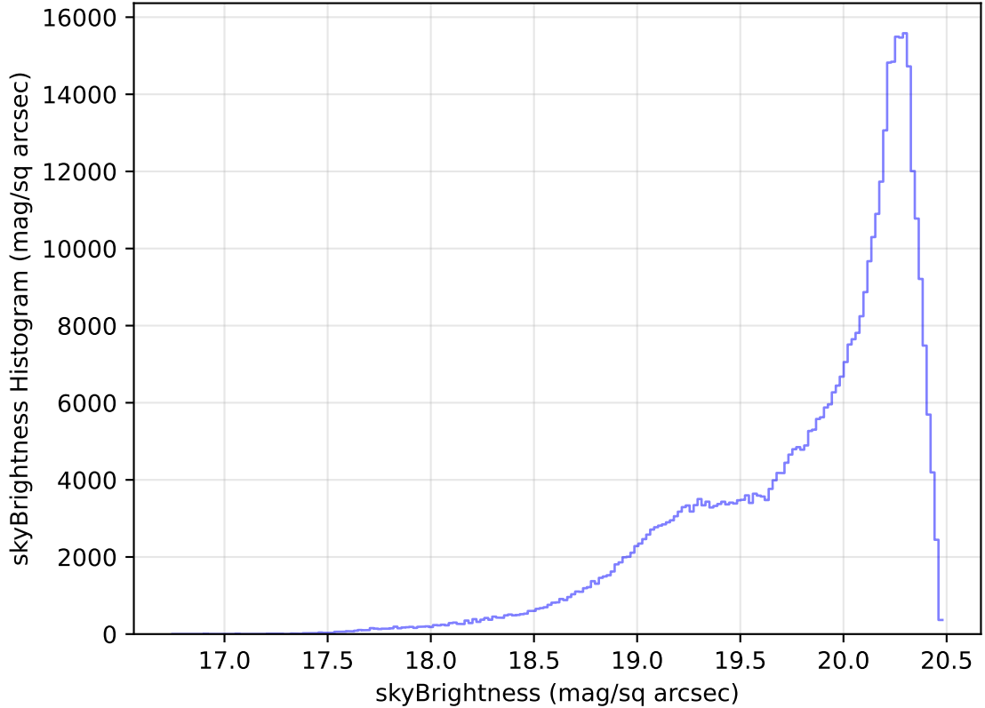
too_elab_heavy_r128_d3_griz_v3.4_10yrs WFD i band: skyBrightness Histogram
