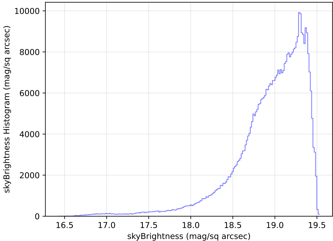
too_elab_heavy_r128_d3_griz_v3.4_10yrs All sky z band: skyBrightness Histogram
