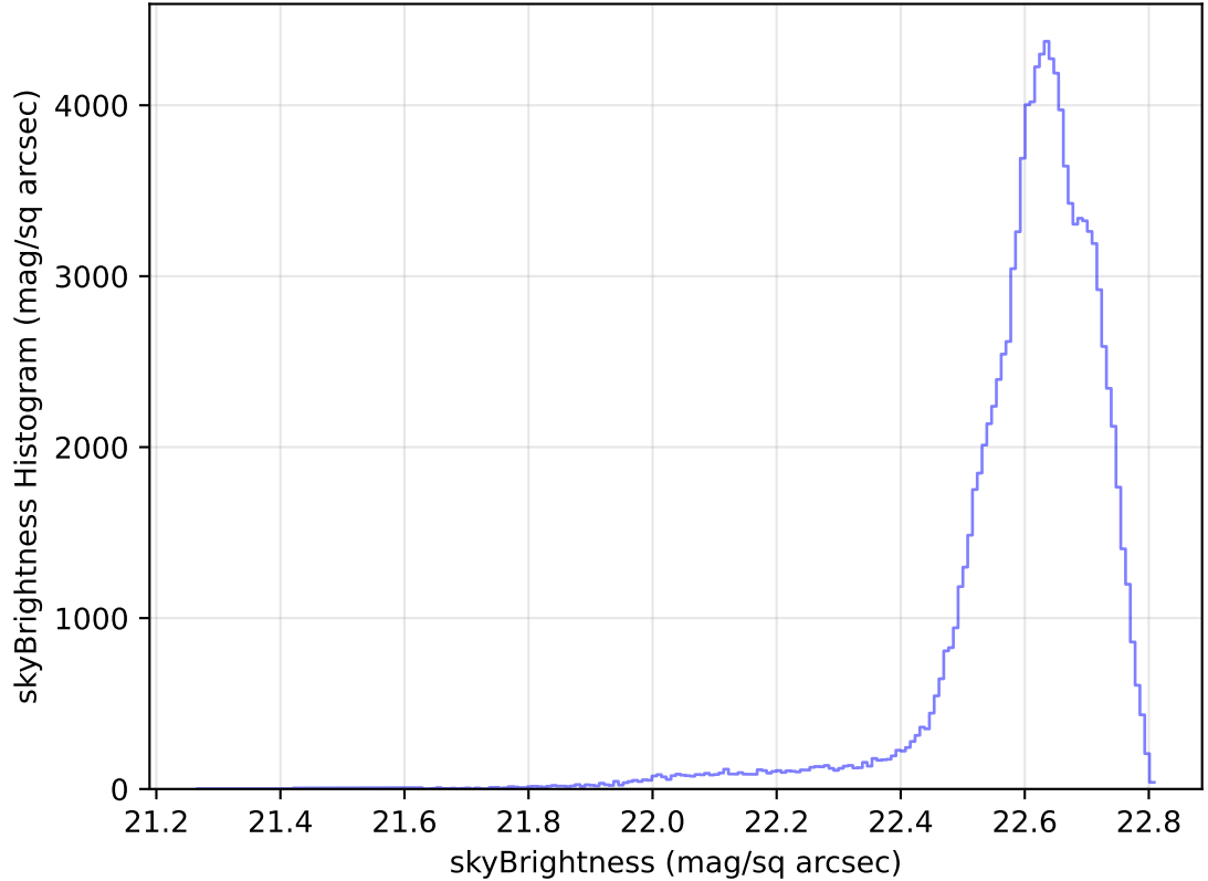
too_elab_heavy_r128_d3_griz_v3.4_10yrs All sky u band: skyBrightness Histogram
