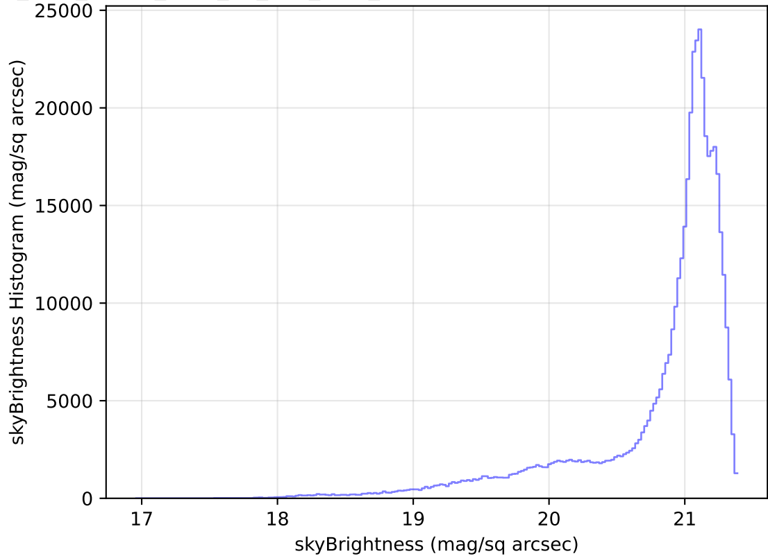
too_elab_heavy_r128_d3_griz_v3.4_10yrs All sky r band: skyBrightness Histogram
