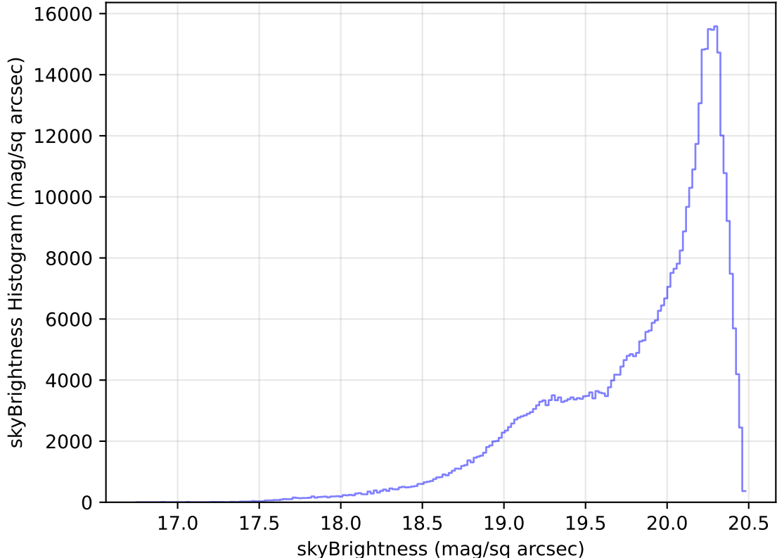
too_elab_heavy_r128_d3_griz_v3.4_10yrs All sky i band: skyBrightness Histogram
