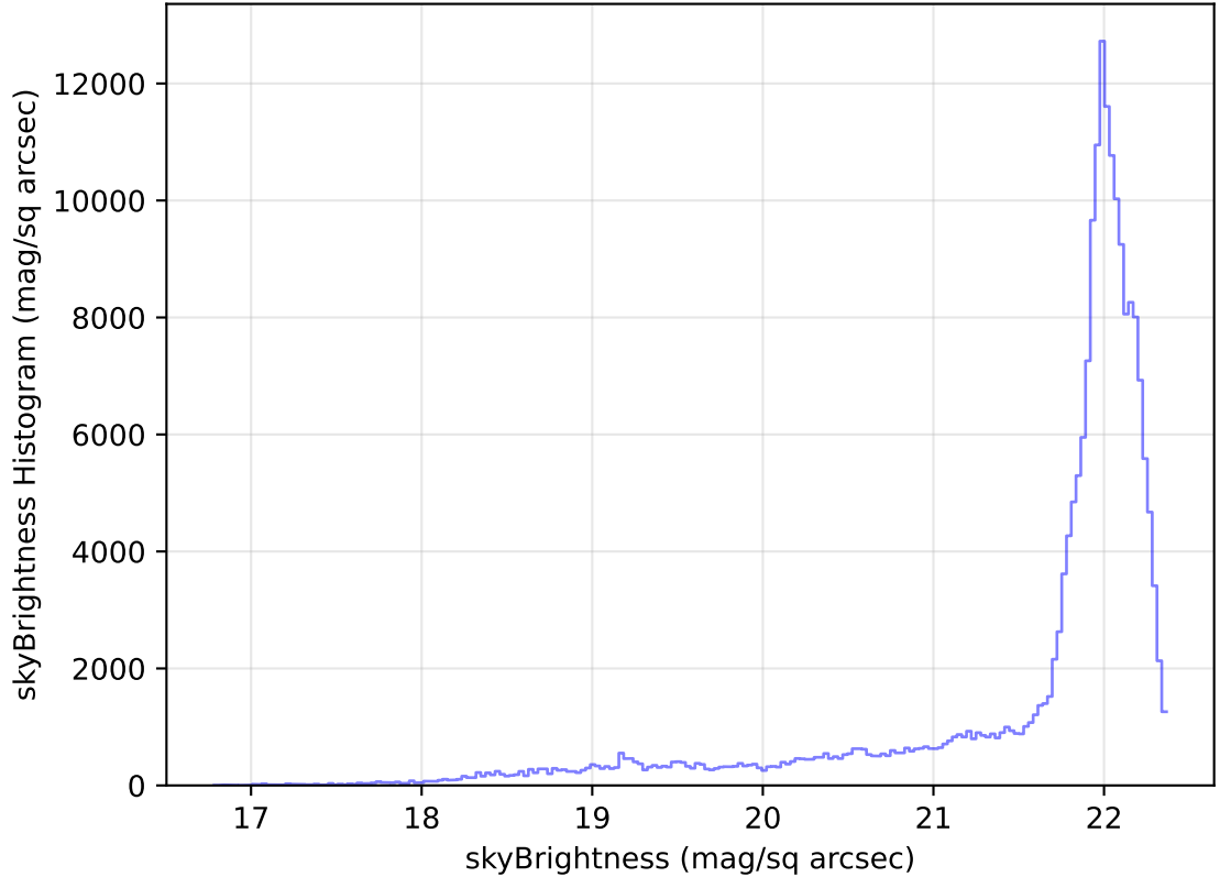
too_elab_heavy_r128_d3_griz_v3.4_10yrs All sky g band: skyBrightness Histogram
