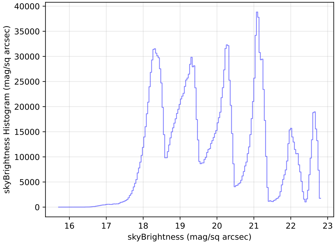
too_elab_heavy_r128_d3_griz_v3.4_10yrs All sky all bands: skyBrightness Histogram
