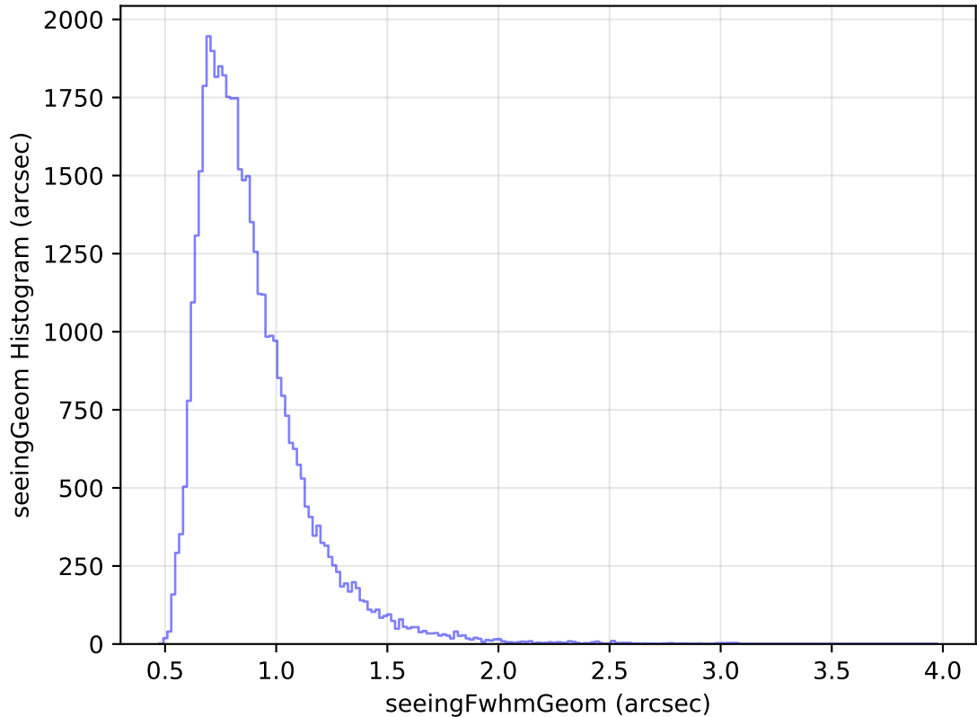
too_elab_heavy_r128_d3_griz_v3.4_10yrs Yr 1 z band: seeingGeom Histogram
