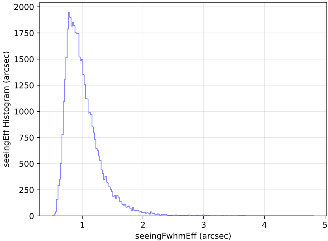
too_elab_heavy_r128_d3_griz_v3.4_10yrs Yr 1 z band: seeingEff Histogram
