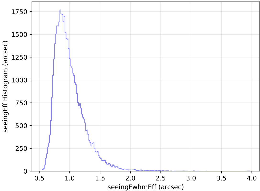
too_elab_heavy_r128_d3_griz_v3.4_10yrs Yr 1 y band: seeingEff Histogram
