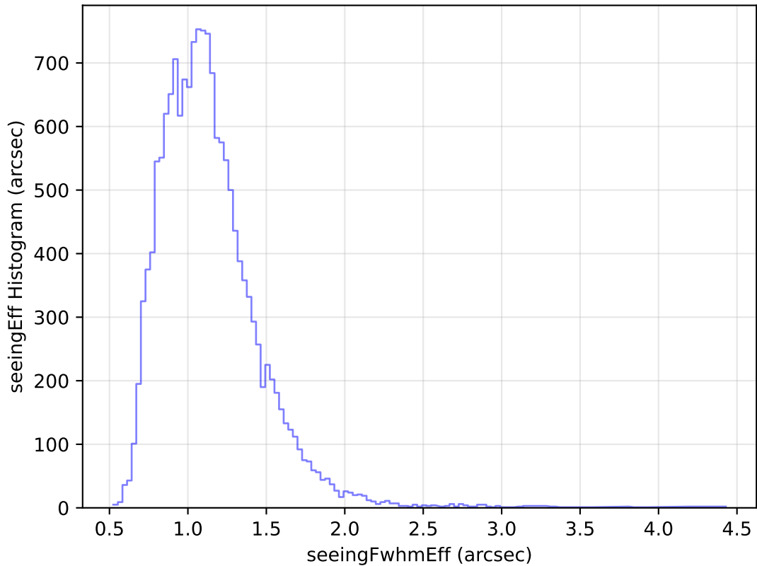
too_elab_heavy_r128_d3_griz_v3.4_10yrs Yr 1 u band: seeingEff Histogram
