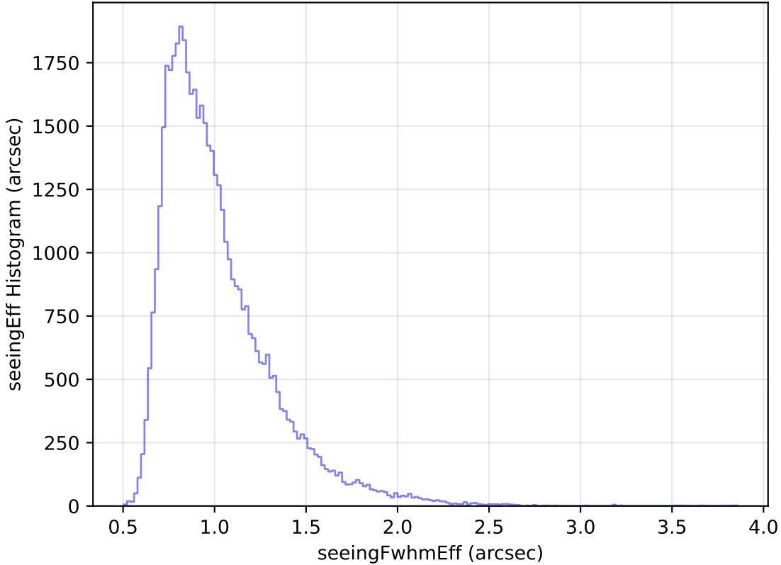
too_elab_heavy_r128_d3_griz_v3.4_10yrs Yr 1 r band: seeingEff Histogram
