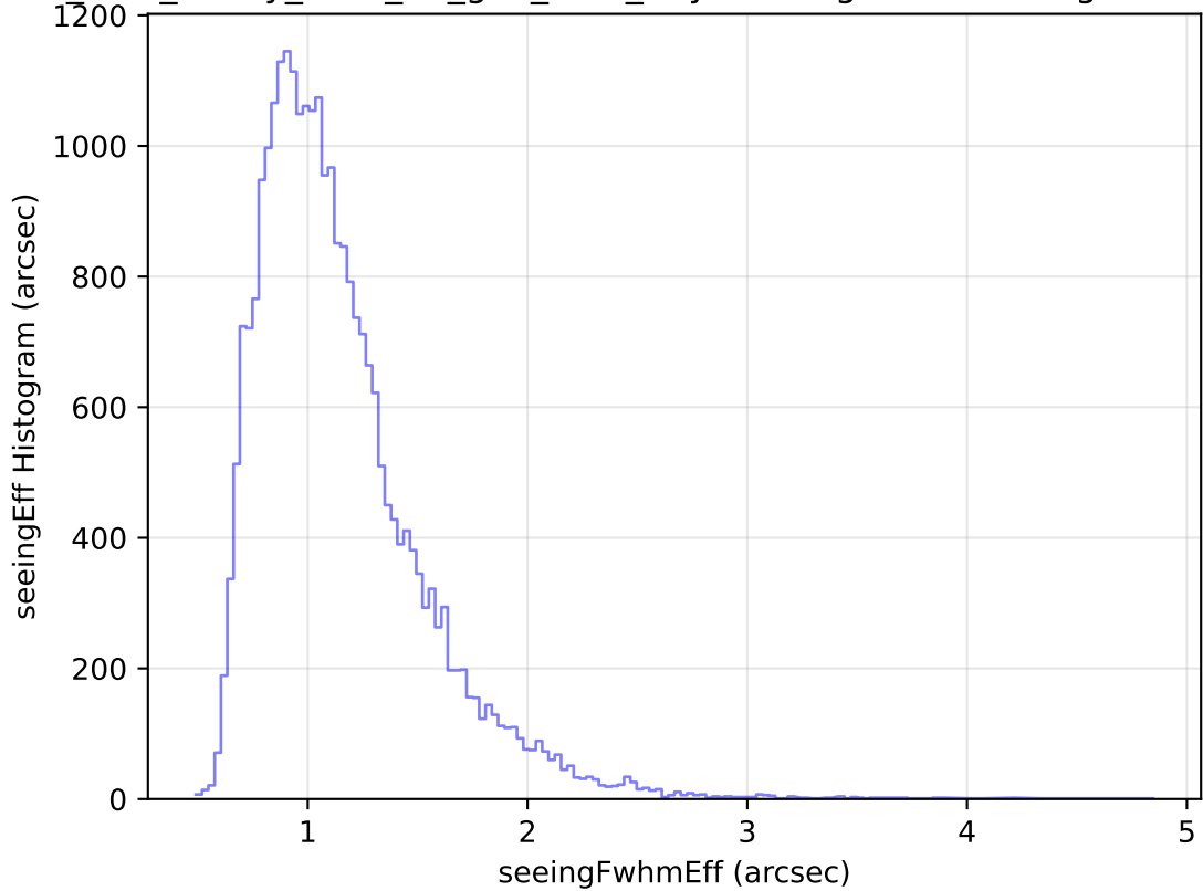
too_elab_heavy_r128_d3_griz_v3.4_10yrs Yr 1 g band: seeingEff Histogram
