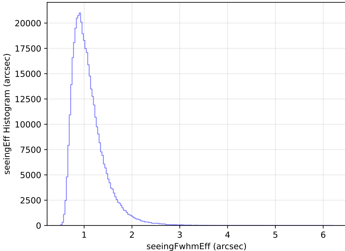
too_elab_heavy_r128_d3_griz_v3.4_10yrs WFD z band: seeingEff Histogram
