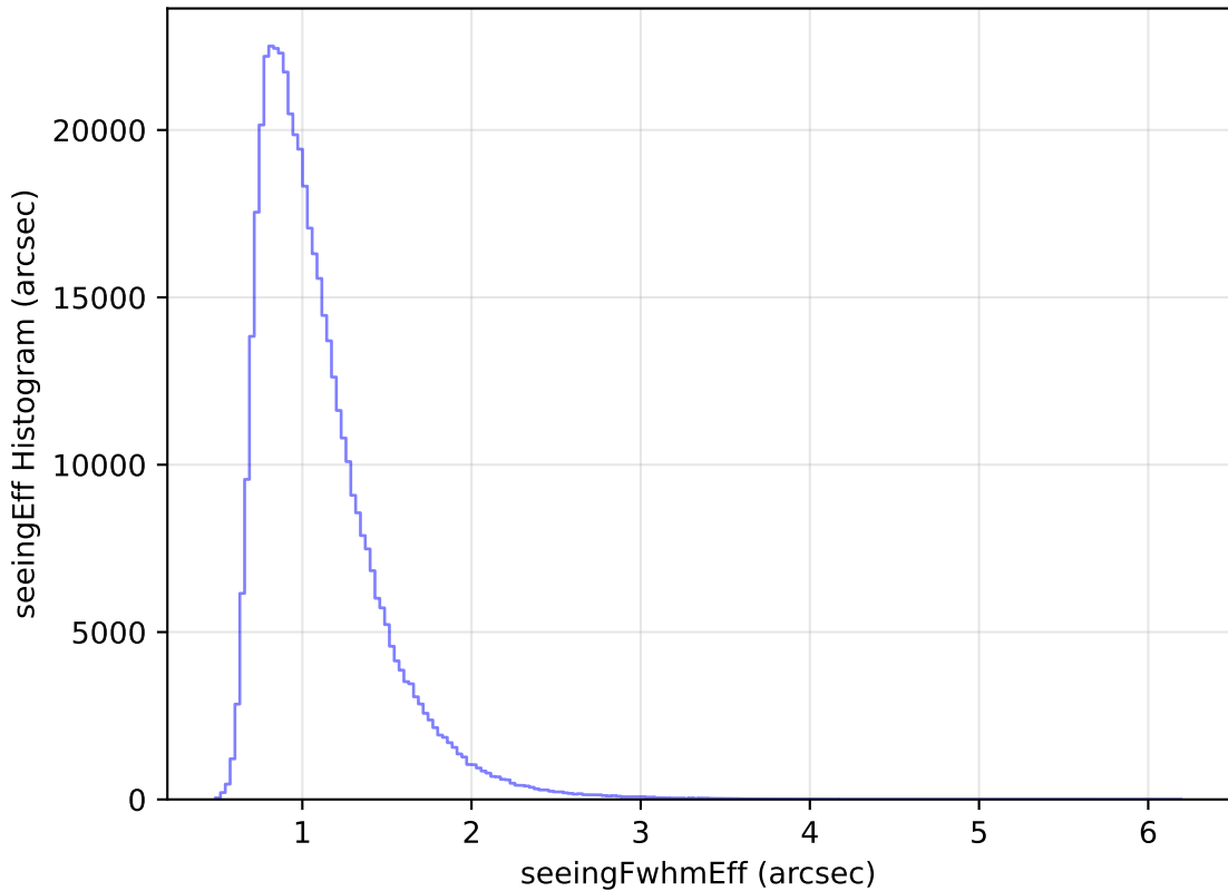
too_elab_heavy_r128_d3_griz_v3.4_10yrs WFD i band: seeingEff Histogram
