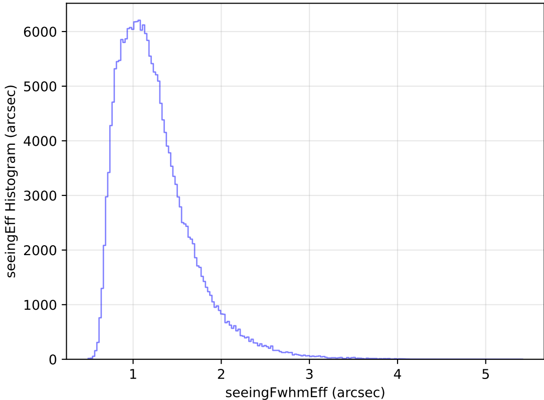
too_elab_heavy_r128_d3_griz_v3.4_10yrs WFD g band: seeingEff Histogram
