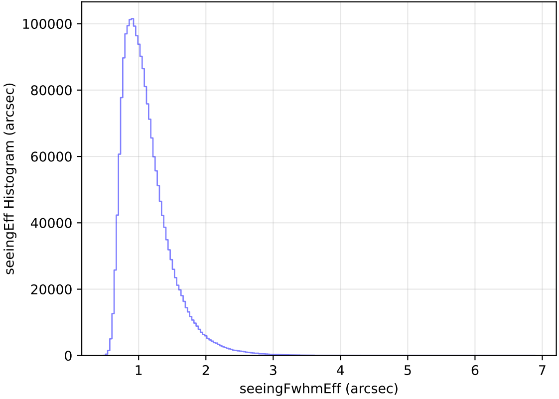
too_elab_heavy_r128_d3_griz_v3.4_10yrs WFD all bands: seeingEff Histogram
