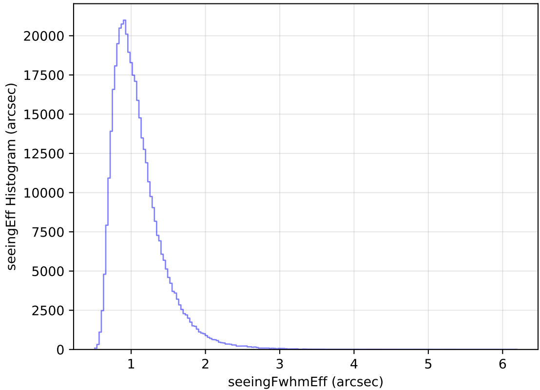
too_elab_heavy_r128_d3_griz_v3.4_10yrs All sky z band: seeingEff Histogram
