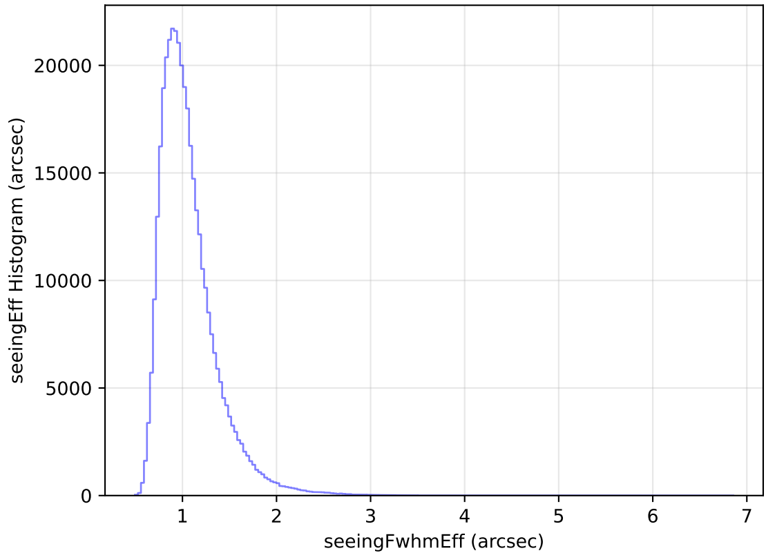
too_elab_heavy_r128_d3_griz_v3.4_10yrs All sky y band: seeingEff Histogram
