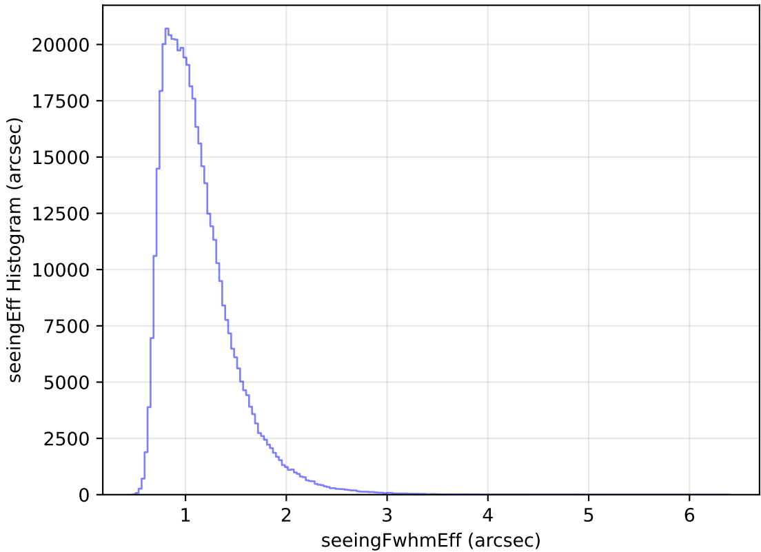
too_elab_heavy_r128_d3_griz_v3.4_10yrs All sky r band: seeingEff Histogram
