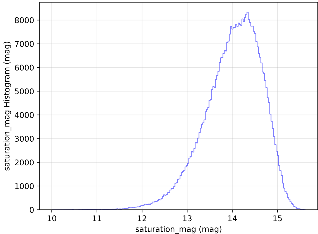
too_elab_heavy_r128_d3_griz_v3.4_10yrs WFD z band: saturation_mag Histogram
