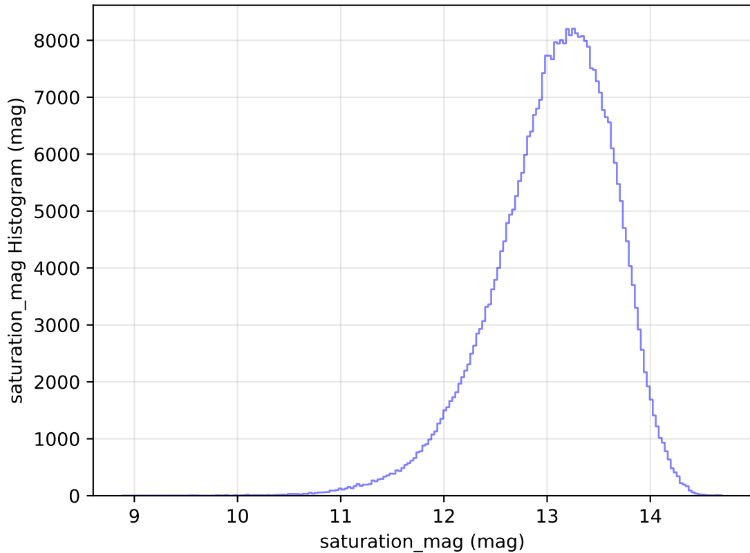
too_elab_heavy_r128_d3_griz_v3.4_10yrs WFD y band: saturation_mag Histogram
