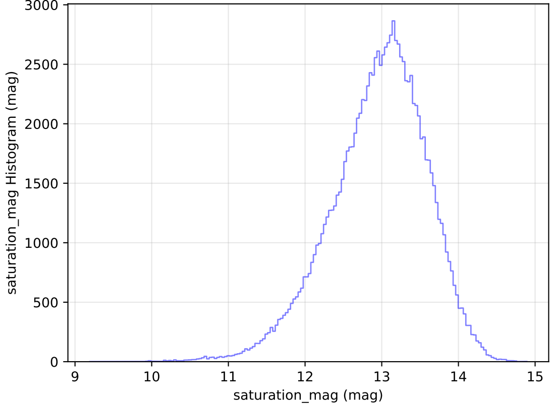
too_elab_heavy_r128_d3_griz_v3.4_10yrs WFD u band: saturation_mag Histogram
