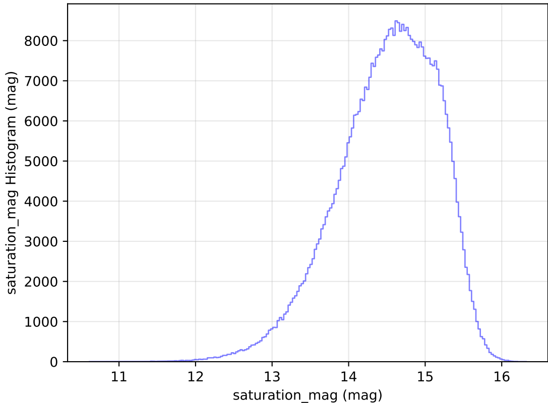
too_elab_heavy_r128_d3_griz_v3.4_10yrs WFD r band: saturation_mag Histogram
