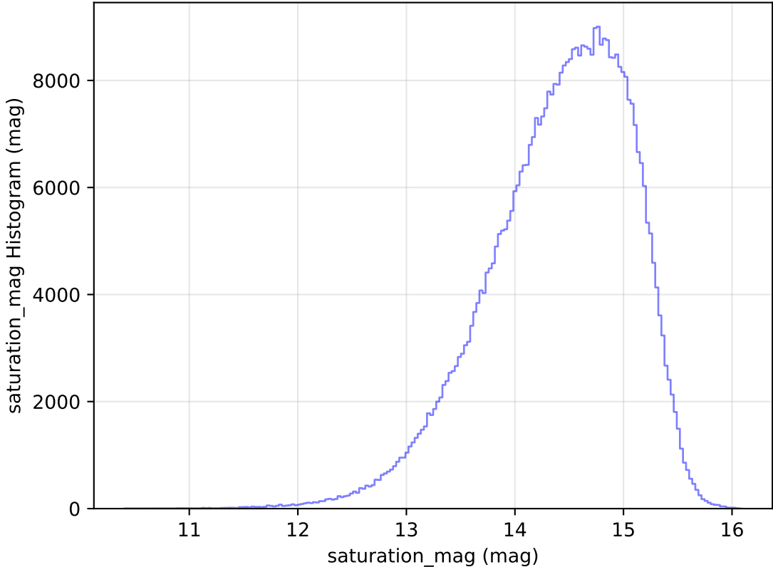
too_elab_heavy_r128_d3_griz_v3.4_10yrs WFD i band: saturation_mag Histogram
