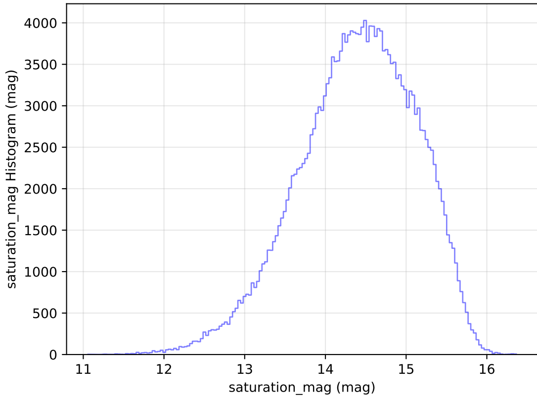
too_elab_heavy_r128_d3_griz_v3.4_10yrs WFD g band: saturation_mag Histogram
