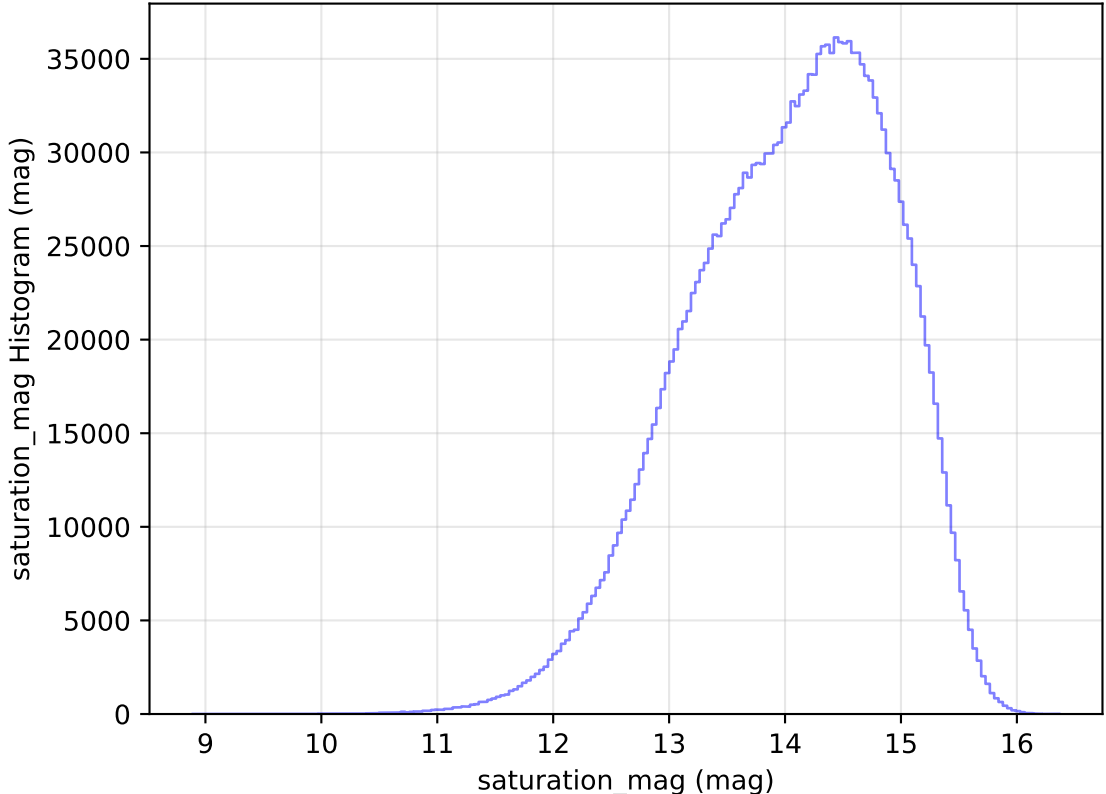
too_elab_heavy_r128_d3_griz_v3.4_10yrs WFD all bands: saturation_mag Histogram
