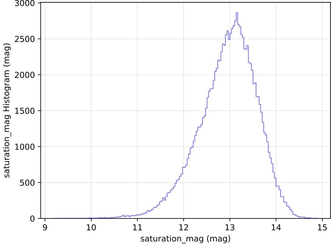
too_elab_heavy_r128_d3_griz_v3.4_10yrs All sky u band: saturation_mag Histogram
