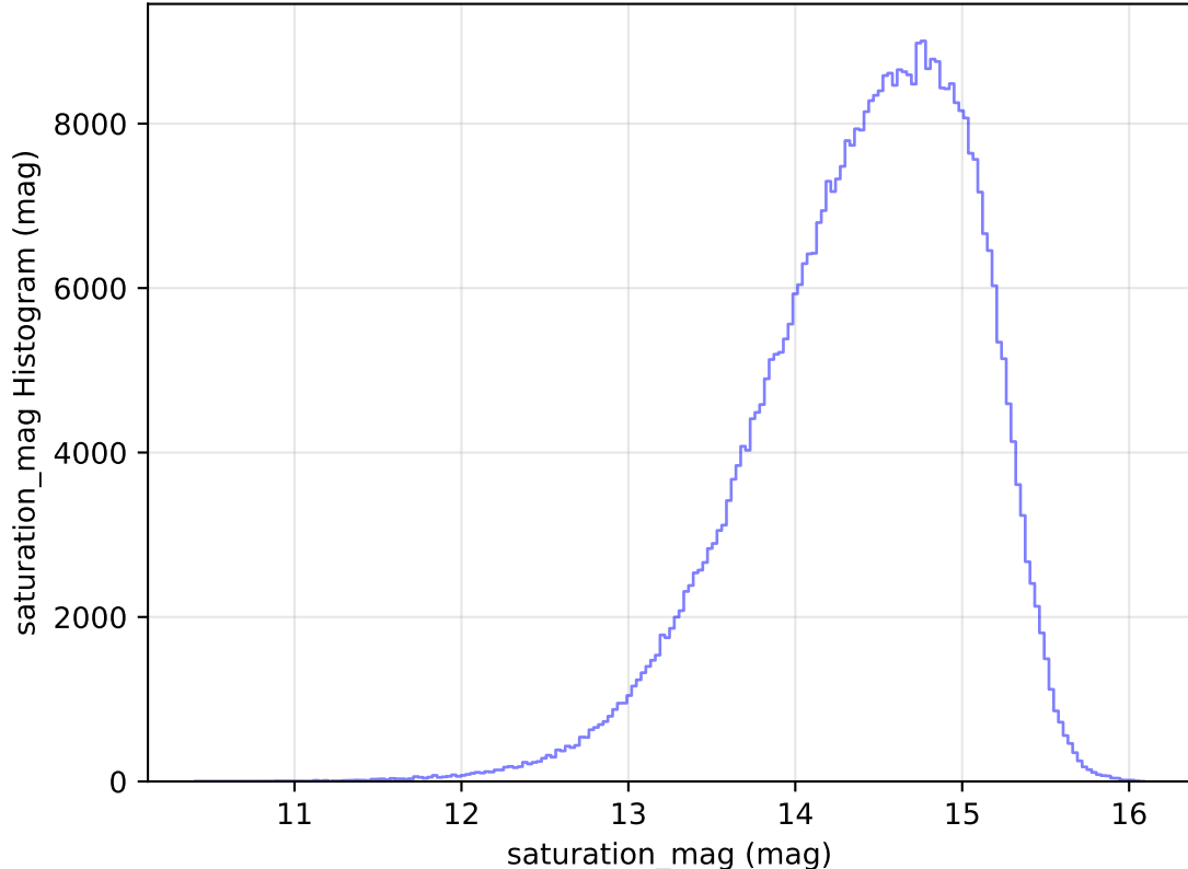
too_elab_heavy_r128_d3_griz_v3.4_10yrs All sky i band: saturation_mag Histogram
